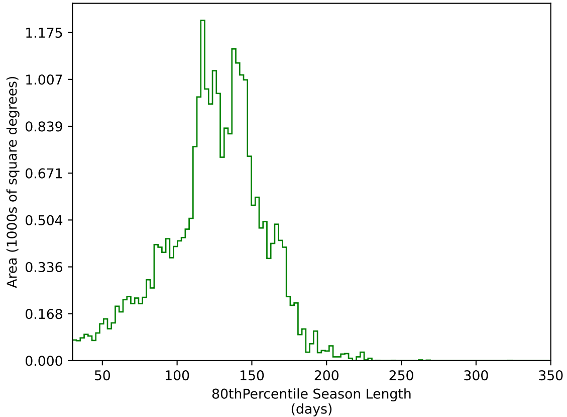
too_elab_heavy_r128_d2_ugrizy_v3.4_10yrs All sky g band: 80thPercentile Season Length
