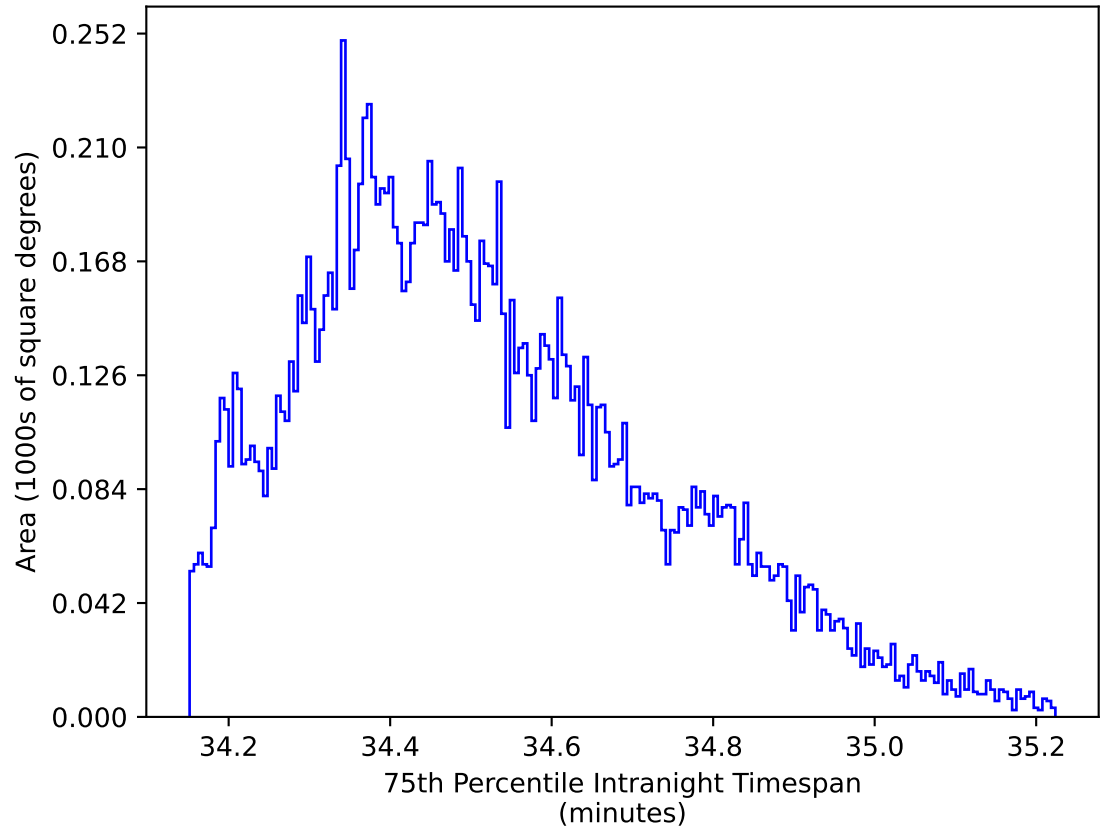
too_elab_heavy_r128_d2_ugrizy_v3.4_10yrs WFD zy bands: 75th Percentile Intranight Timespan
