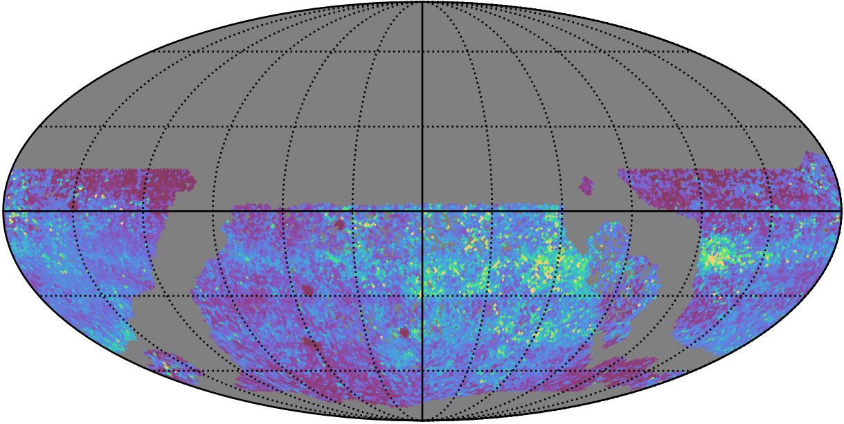
too_elab_heavy_r128_d2_ugrizy_v3.4_10yrs WFD y band: 75th Percentile Intranight Timespan
