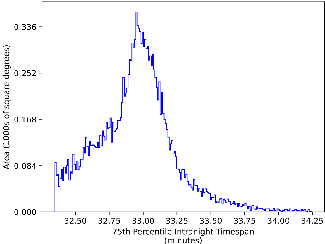
too_elab_heavy_r128_d2_ugrizy_v3.4_10yrs WFD y band: 75th Percentile Intranight Timespan
