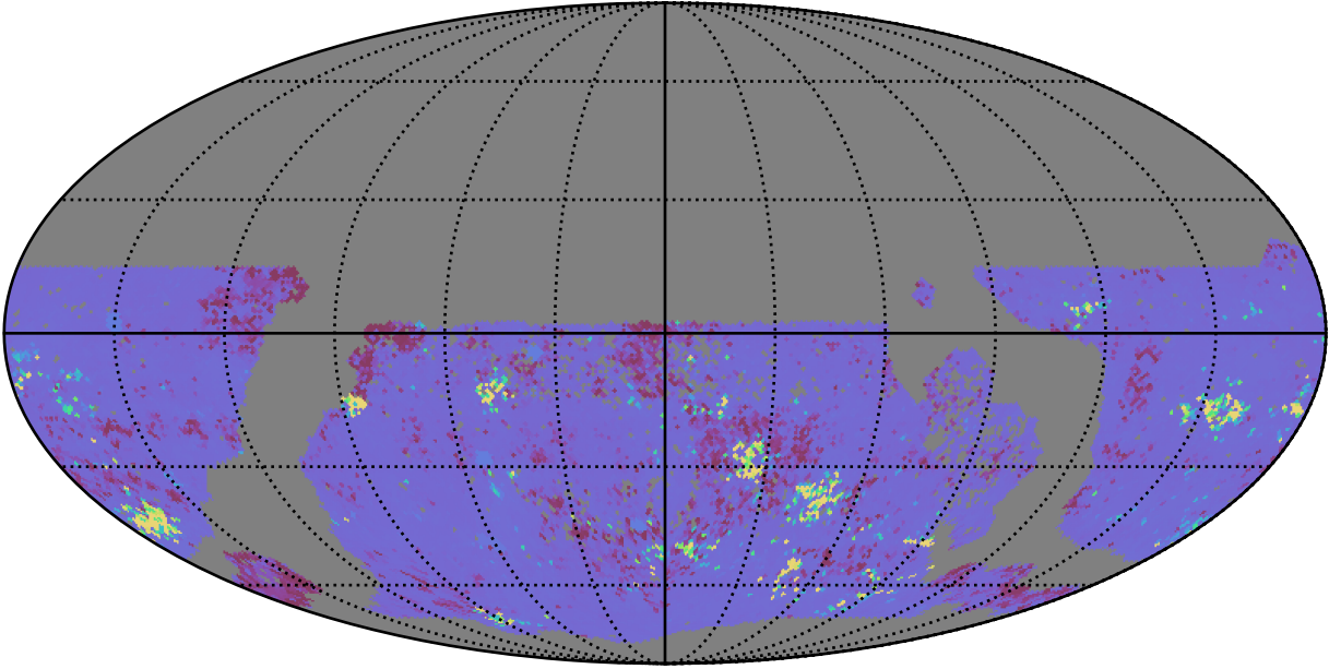
too_elab_heavy_r128_d2_ugrizy_v3.4_10yrs WFD ug bands: 75th Percentile Intranight Timespan
