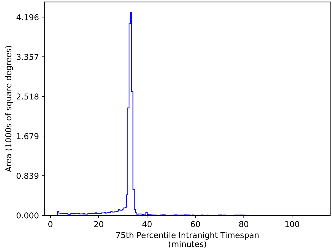
too_elab_heavy_r128_d2_ugrizy_v3.4_10yrs WFD ug bands: 75th Percentile Intranight Timespan
