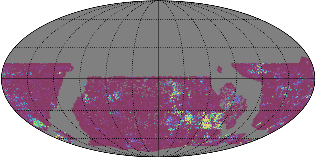
too_elab_heavy_r128_d2_ugrizy_v3.4_10yrs WFD u band: 75th Percentile Intranight Timespan
