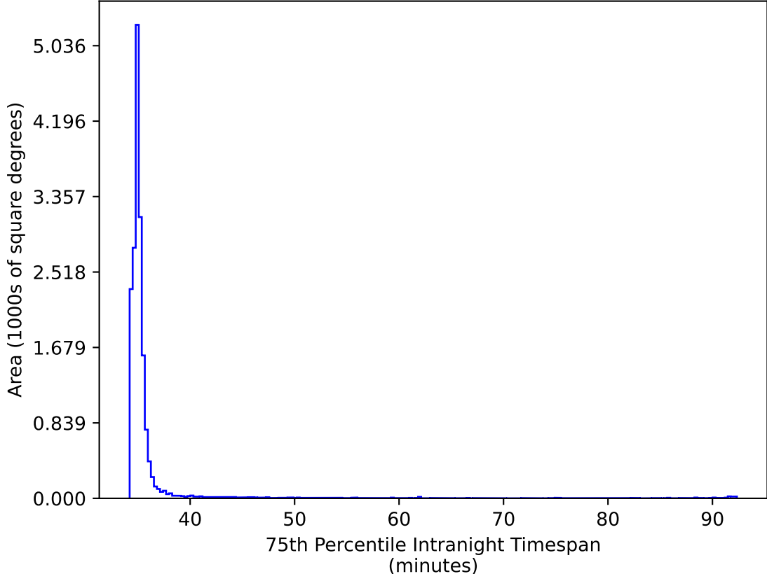
too_elab_heavy_r128_d2_ugrizy_v3.4_10yrs WFD ri bands: 75th Percentile Intranight Timespan
