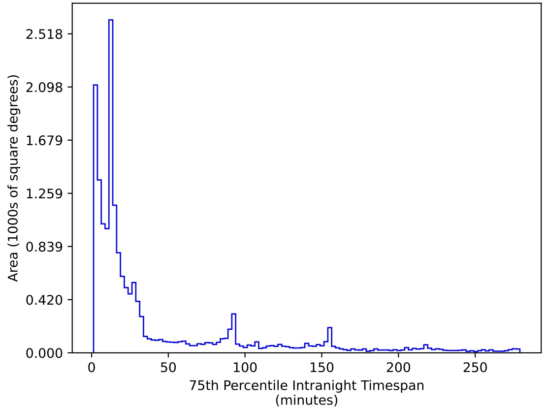
too_elab_heavy_r128_d2_ugrizy_v3.4_10yrs WFD r band: 75th Percentile Intranight Timespan
