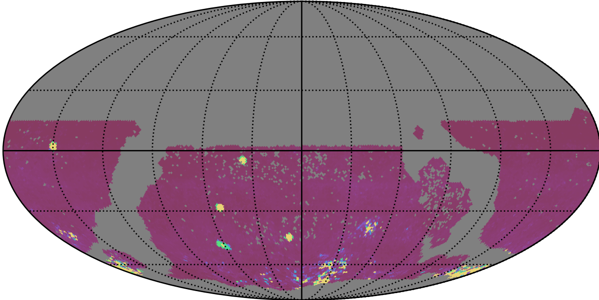
too_elab_heavy_r128_d2_ugrizy_v3.4_10yrs WFD iz bands: 75th Percentile Intranight Timespan
