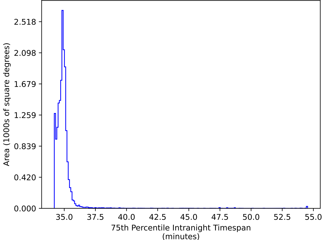
too_elab_heavy_r128_d2_ugrizy_v3.4_10yrs WFD iz bands: 75th Percentile Intranight Timespan
