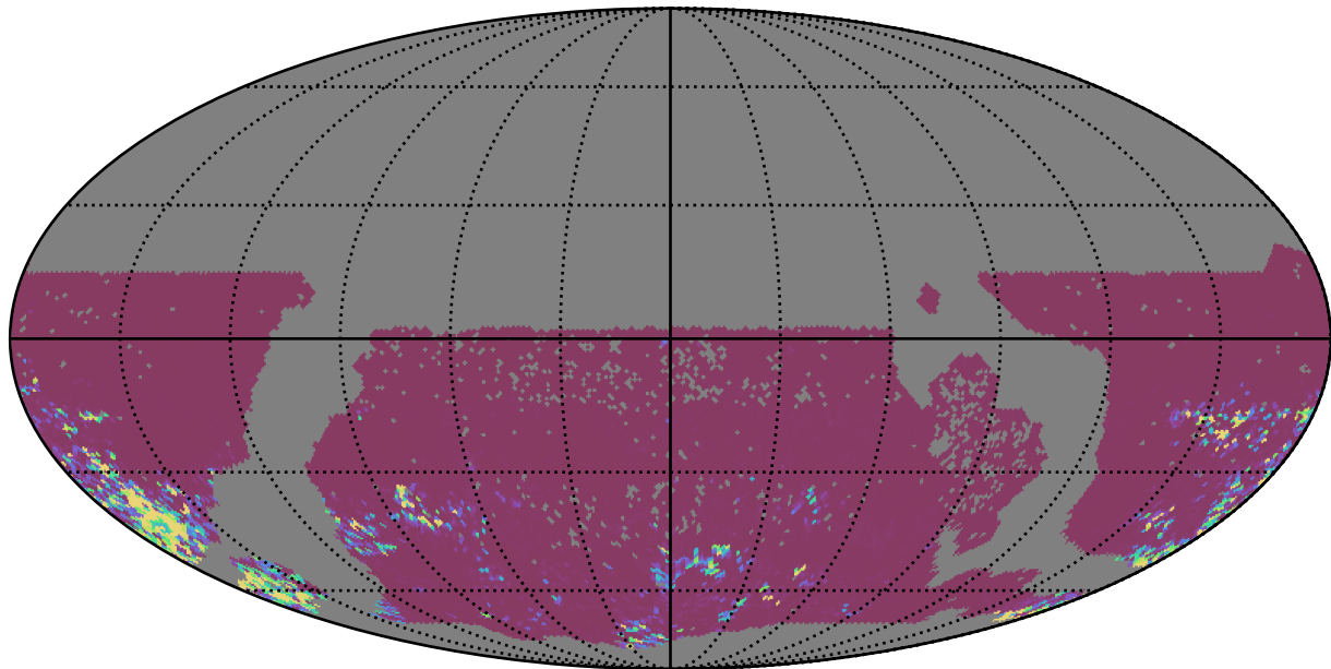
too_elab_heavy_r128_d2_ugrizy_v3.4_10yrs WFD gr bands: 75th Percentile Intranight Timespan
