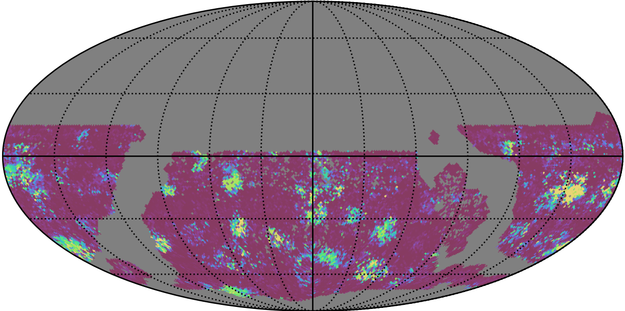
too_elab_heavy_r128_d2_ugrizy_v3.4_10yrs WFD g band: 75th Percentile Intranight Timespan
