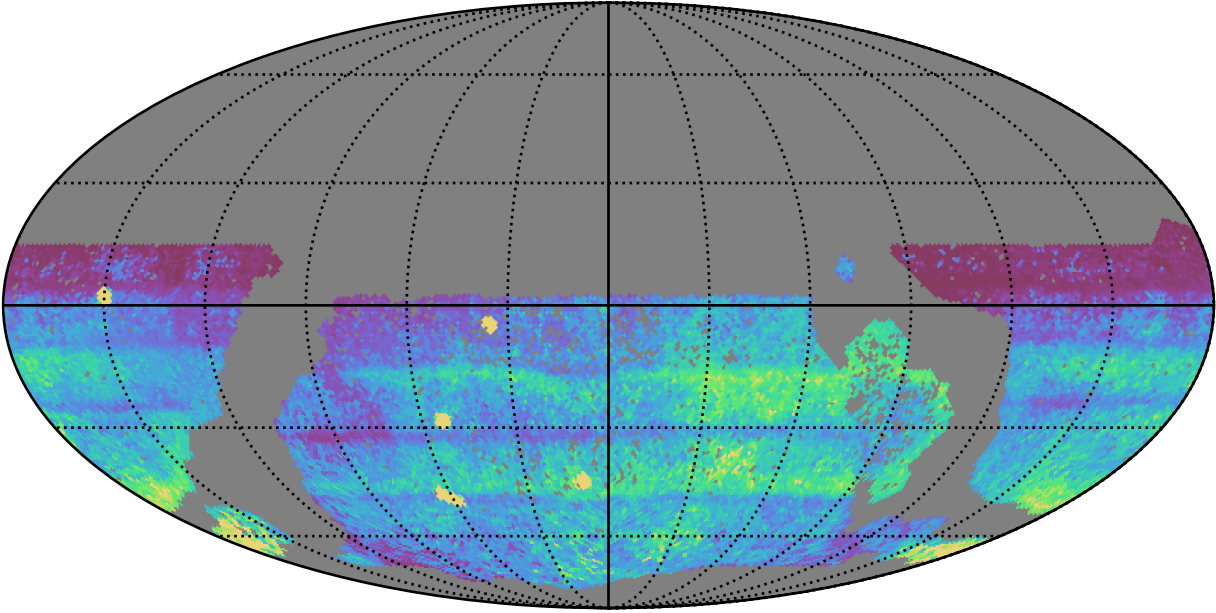
too_elab_heavy_r128_d2_ugrizy_v3.4_10yrs WFD all bands: 75th Percentile Intranight Timespan
