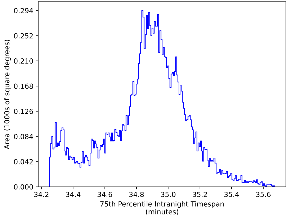
too_elab_heavy_r128_d2_ugrizy_v3.4_10yrs WFD all bands: 75th Percentile Intranight Timespan
