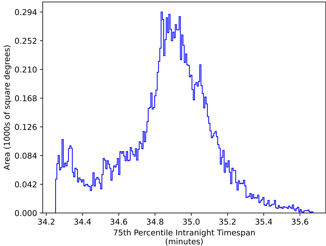
too_elab_heavy_r128_d2_ugrizy_v3.4_10yrs WFD: 75th Percentile Intranight Timespan
