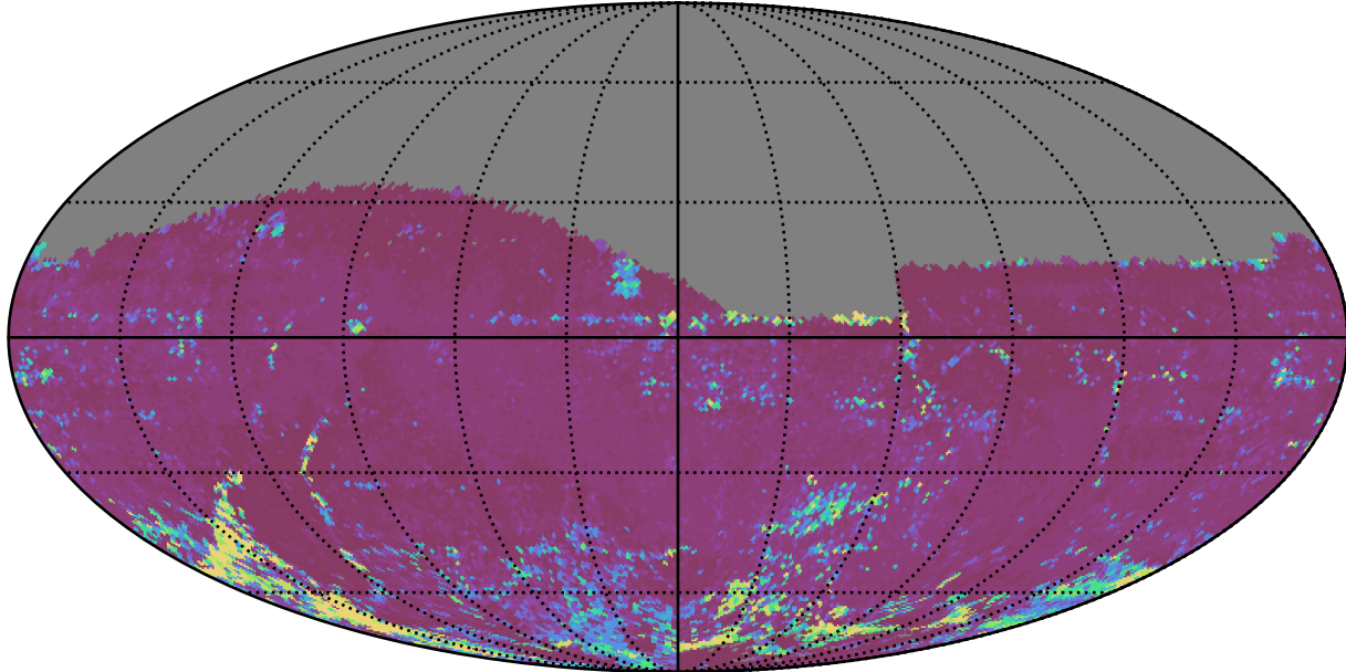
too_elab_heavy_r128_d2_ugrizy_v3.4_10yrs All sky z band: 75th Percentile Intranight Timespan
