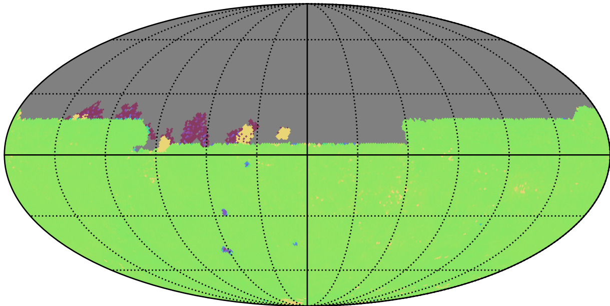
too_elab_heavy_r128_d2_ugrizy_v3.4_10yrs All sky y band: 75th Percentile Intranight Timespan
