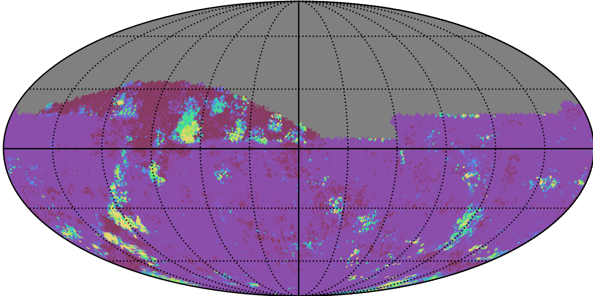
too_elab_heavy_r128_d2_ugrizy_v3.4_10yrs All sky ug bands: 75th Percentile Intranight Timespan
