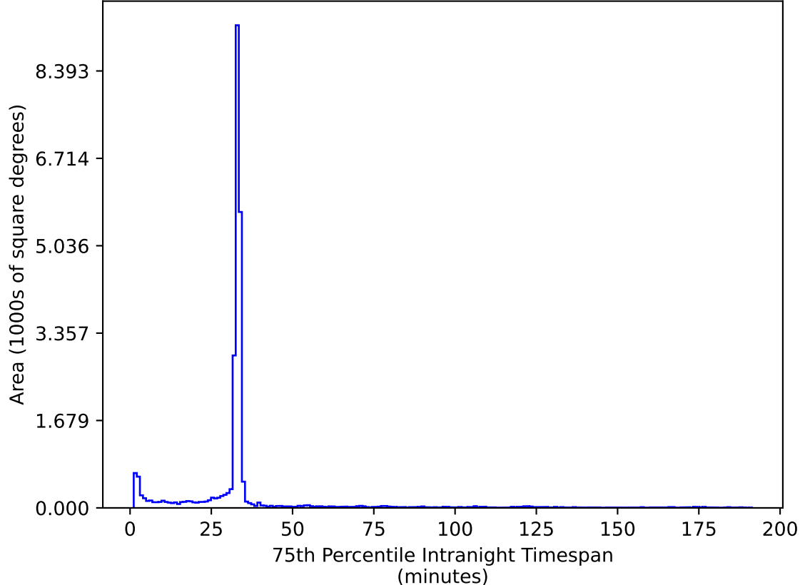
too_elab_heavy_r128_d2_ugrizy_v3.4_10yrs All sky ug bands: 75th Percentile Intranight Timespan
