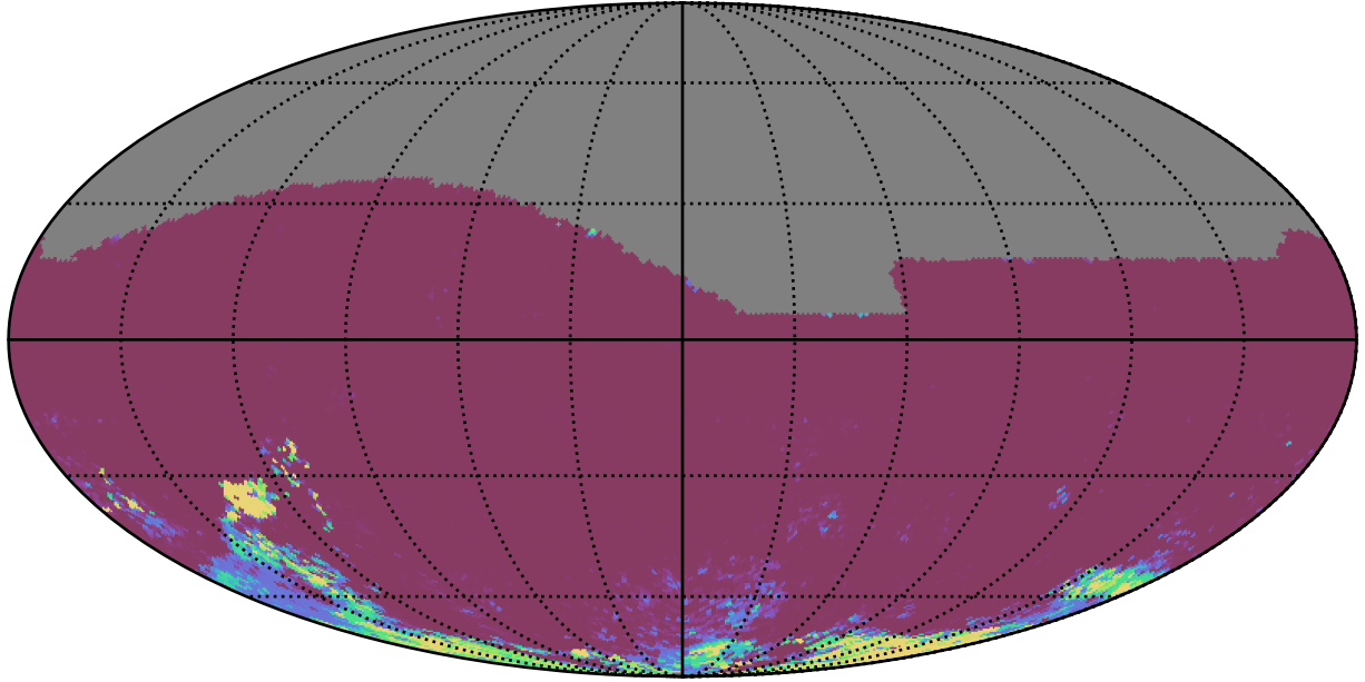
too_elab_heavy_r128_d2_ugrizy_v3.4_10yrs All sky ri bands: 75th Percentile Intranight Timespan
