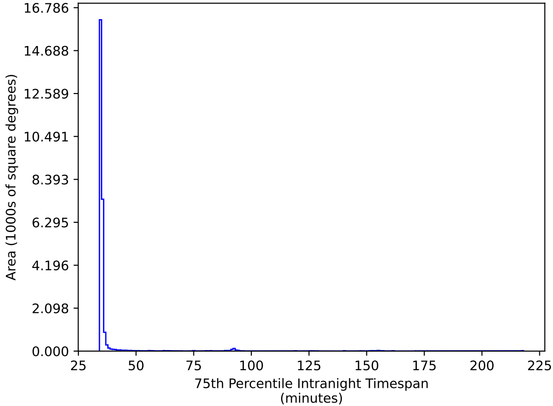
too_elab_heavy_r128_d2_ugrizy_v3.4_10yrs All sky ri bands: 75th Percentile Intranight Timespan
