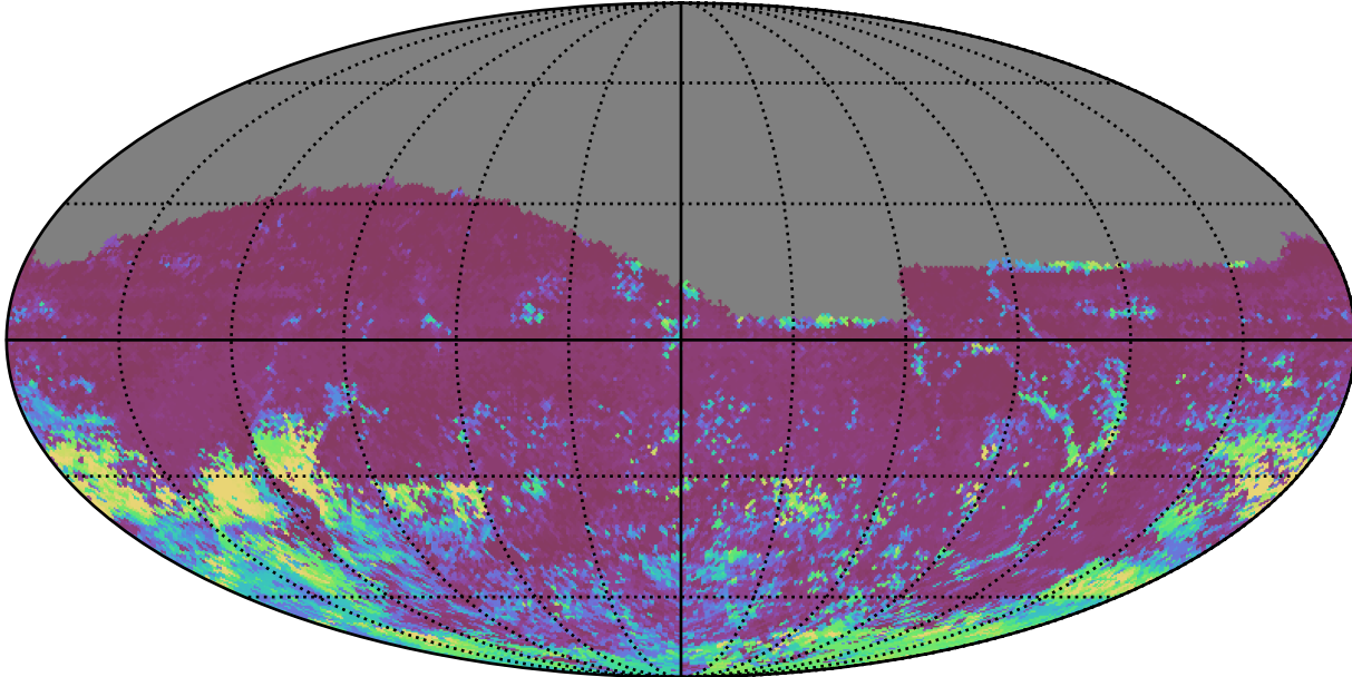
too_elab_heavy_r128_d2_ugrizy_v3.4_10yrs All sky r band: 75th Percentile Intranight Timespan
