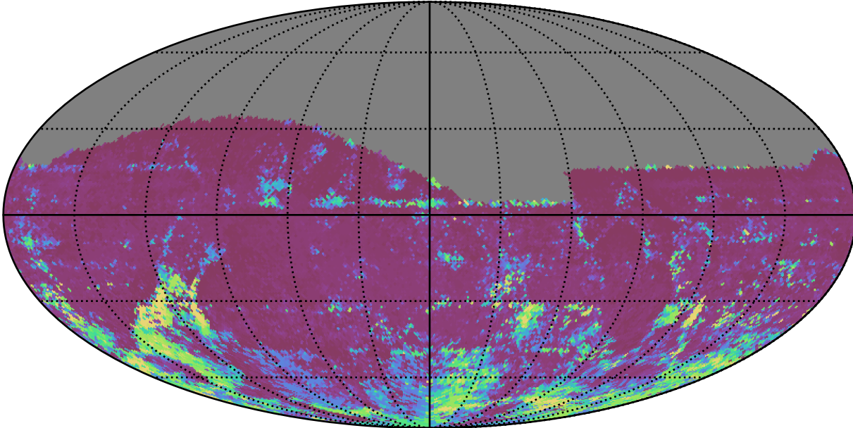
too_elab_heavy_r128_d2_ugrizy_v3.4_10yrs All sky i band: 75th Percentile Intranight Timespan
