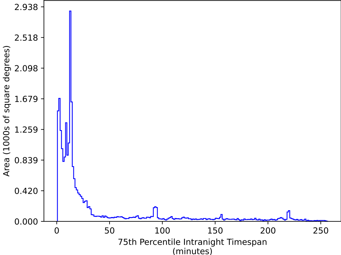
too_elab_heavy_r128_d2_ugrizy_v3.4_10yrs All sky i band: 75th Percentile Intranight Timespan
