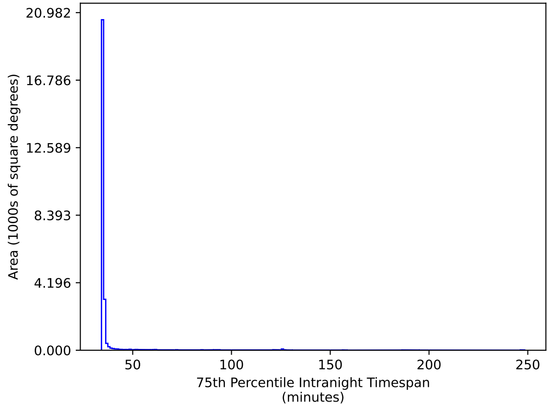
too_elab_heavy_r128_d2_ugrizy_v3.4_10yrs All sky gr bands: 75th Percentile Intranight Timespan
