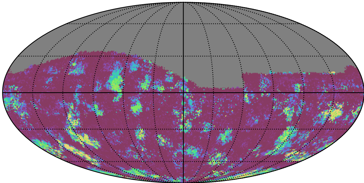
too_elab_heavy_r128_d2_ugrizy_v3.4_10yrs All sky g band: 75th Percentile Intranight Timespan
