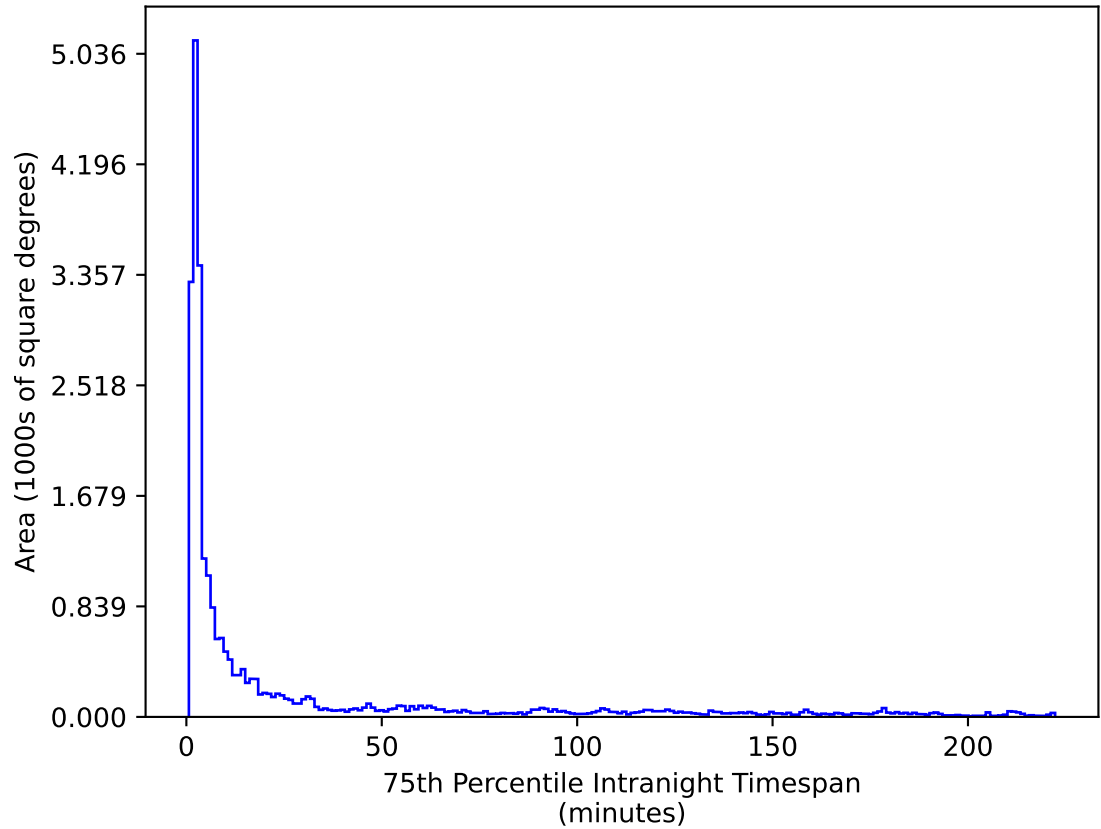
too_elab_heavy_r128_d2_ugrizy_v3.4_10yrs All sky g band: 75th Percentile Intranight Timespan
