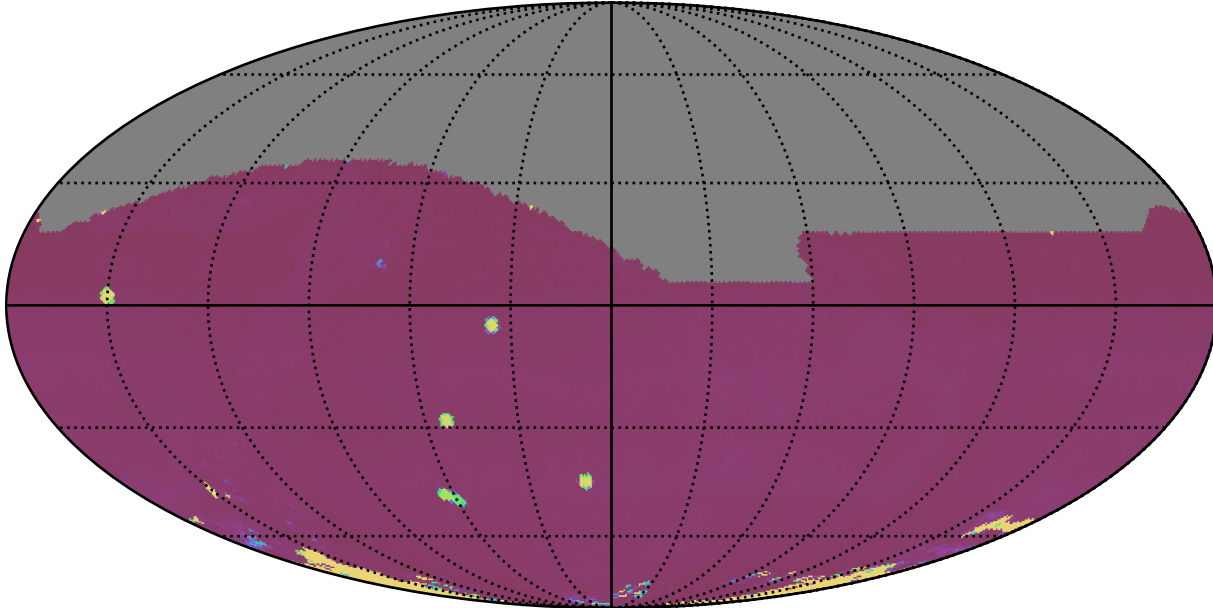
too_elab_heavy_r128_d2_ugrizy_v3.4_10yrs All sky all bands: 75th Percentile Intranight Timespan
