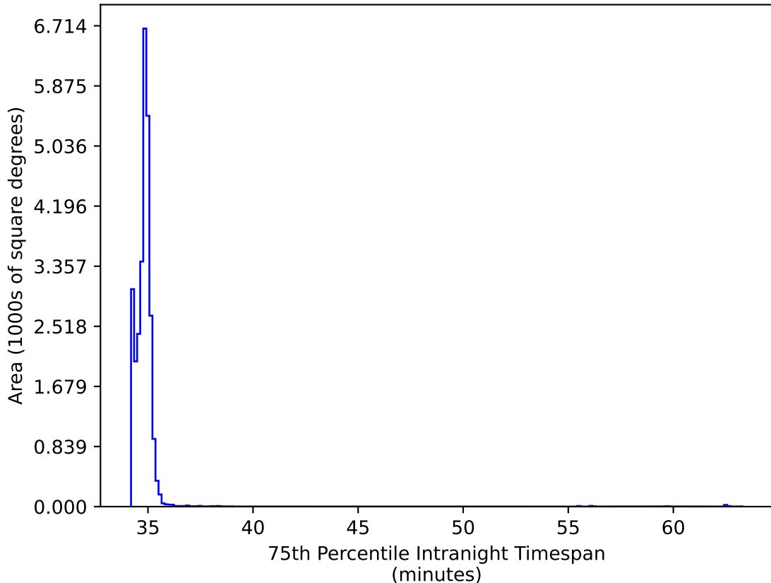
too_elab_heavy_r128_d2_ugrizy_v3.4_10yrs All sky all bands: 75th Percentile Intranight Timespan
