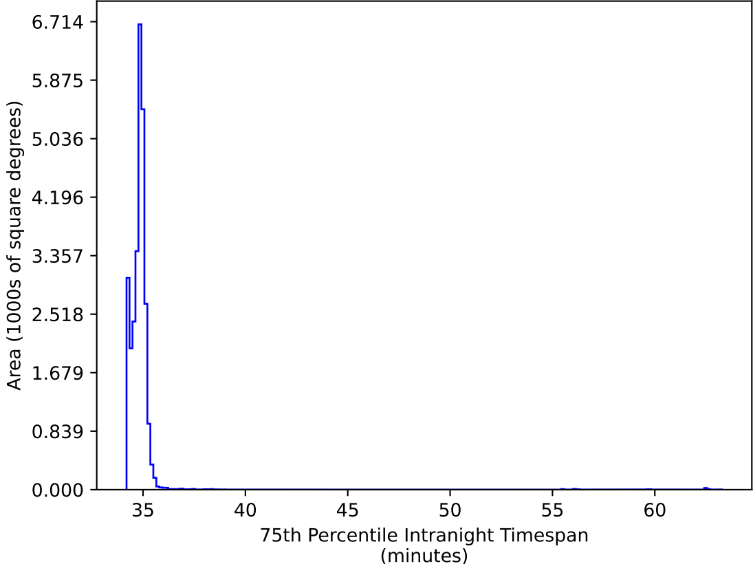
too_elab_heavy_r128_d2_ugrizy_v3.4_10yrs All sky: 75th Percentile Intranight Timespan
