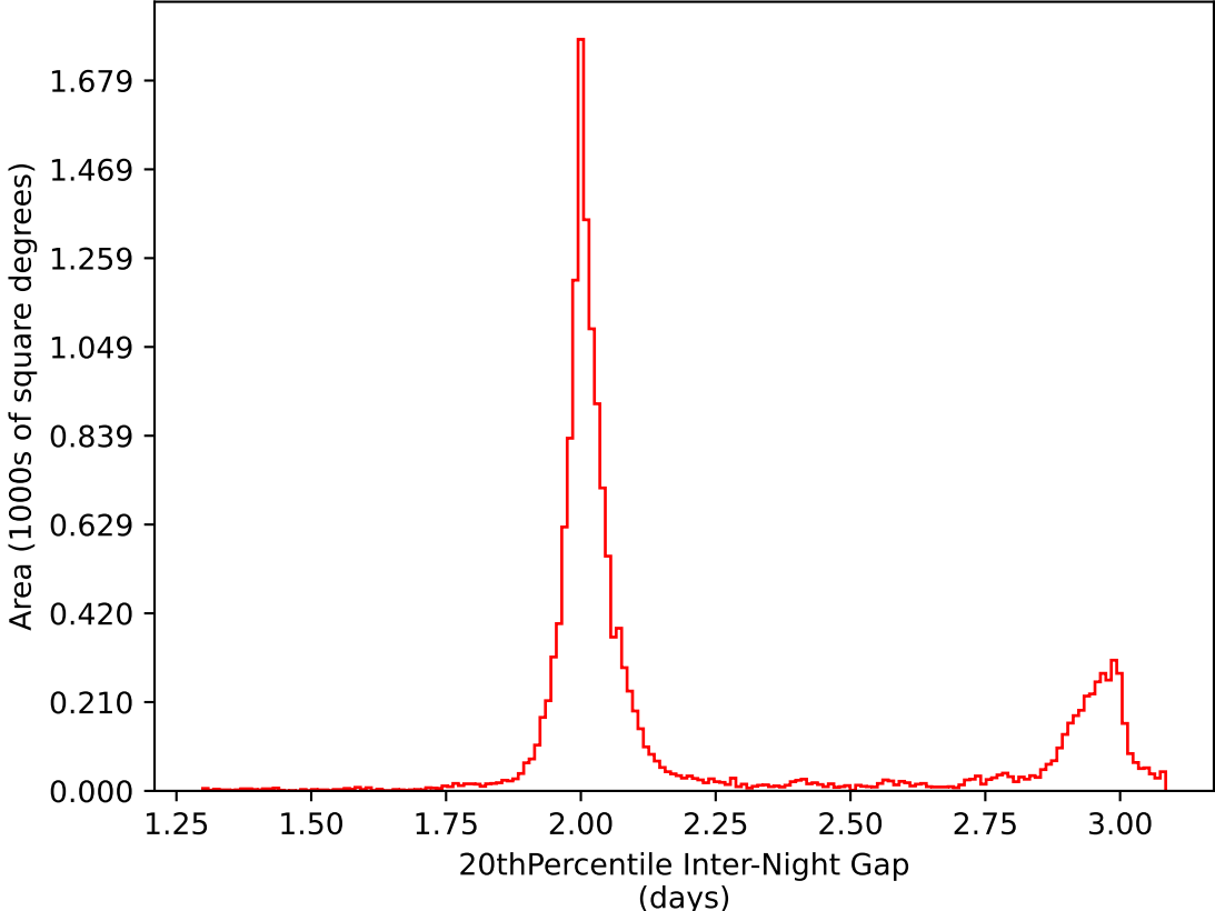
too_elab_heavy_r128_d2_ugrizy_v3.4_10yrs WFD i band: 20thPercentile Inter-Night Gap
