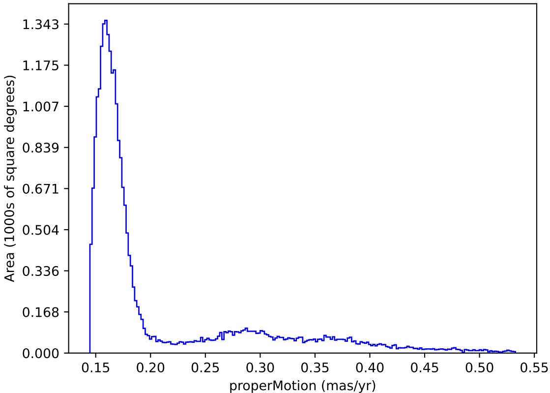
too_elab_heavy_r128_d2_ugrizy_v3.4_10yrs : properMotion
