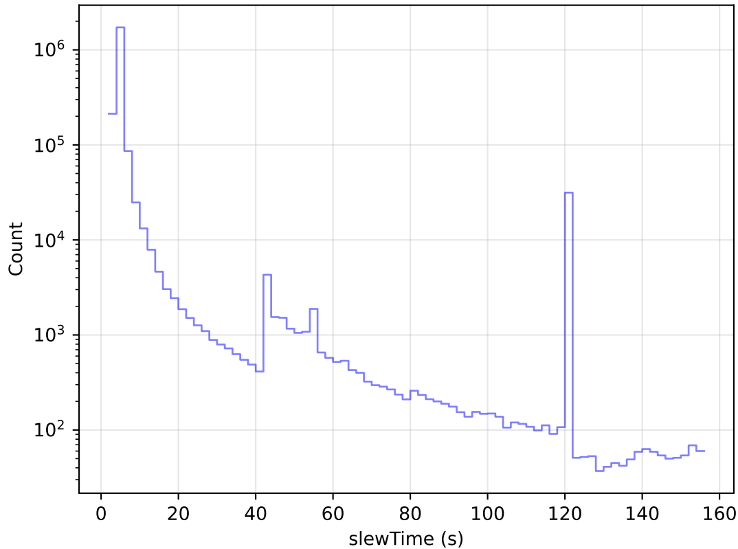
too_elab_heavy_r128_d2_ugrizy_v3.4_10yrs All visits: Slew Time Histogram
