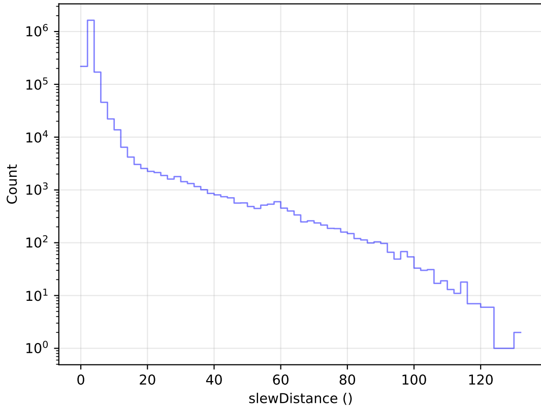
too_elab_heavy_r128_d2_ugrizy_v3.4_10yrs All visits: Slew Distance Histogram
