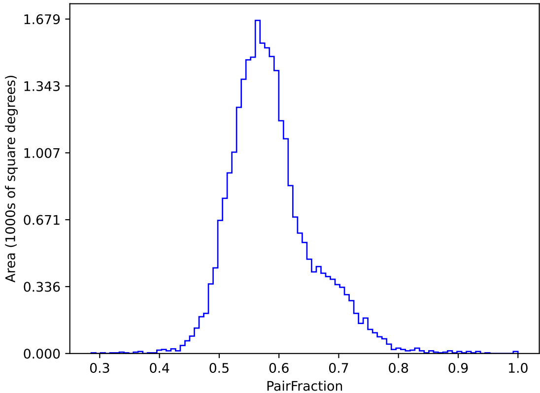
too_elab_heavy_r128_d2_ugrizy_v3.4_10yrs (g or r or i): PairFraction
