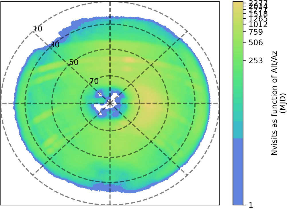
too_elab_heavy_r128_d2_ugrizy_v3.4_10yrs z: Nvisits as function of Alt/Az
