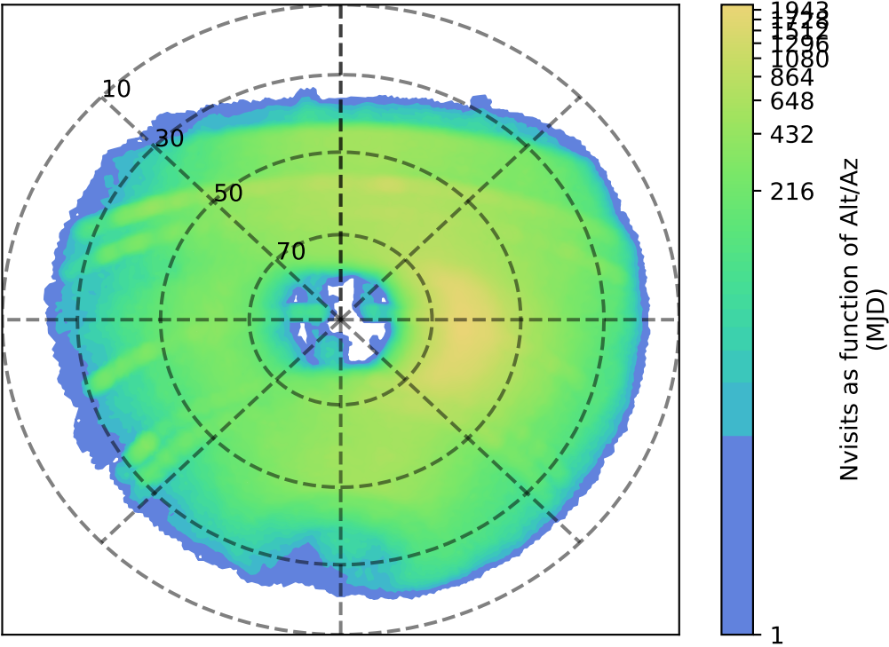
too_elab_heavy_r128_d2_ugrizy_v3.4_10yrs y: Nvisits as function of Alt/Az
