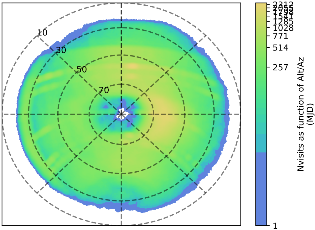
too_elab_heavy_r128_d2_ugrizy_v3.4_10yrs r: Nvisits as function of Alt/Az
