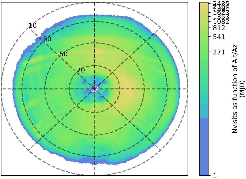
too_elab_heavy_r128_d2_ugrizy_v3.4_10yrs i: Nvisits as function of Alt/Az
