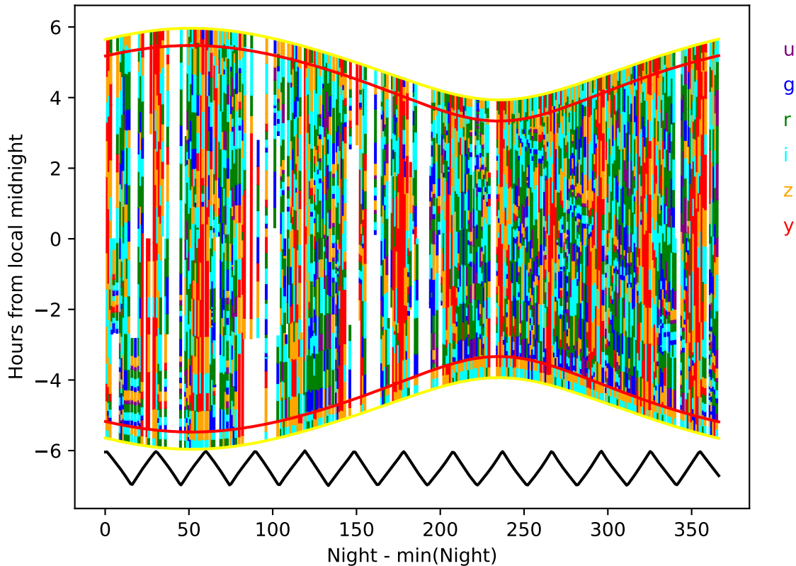
too_elab_heavy_r128_d2_ugrizy_v3.4_10yrs year 1-2: Hourglass
