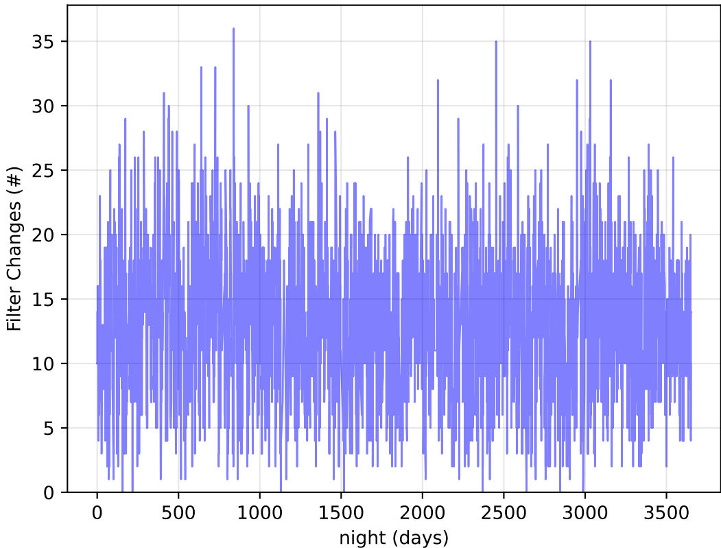
too_elab_heavy_r128_d2_ugrizy_v3.4_10yrs : Filter Changes
