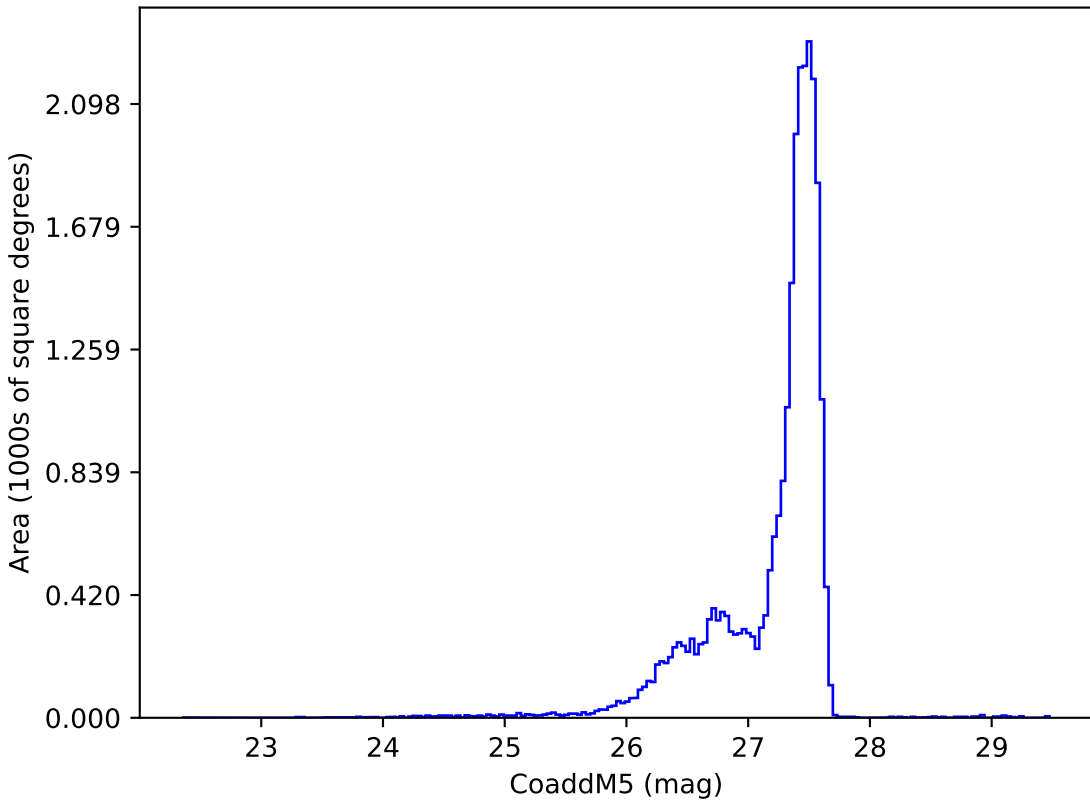
too_elab_heavy_r128_d2_ugrizy_v3.4_10yrs : CoaddM5
