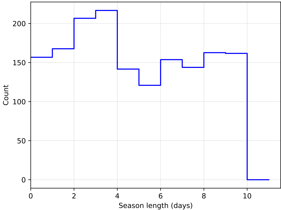
too_elab_heavy_r128_d2_ugrizy_v3.4_10yrs DD:WFD all bands: SeasonLength
