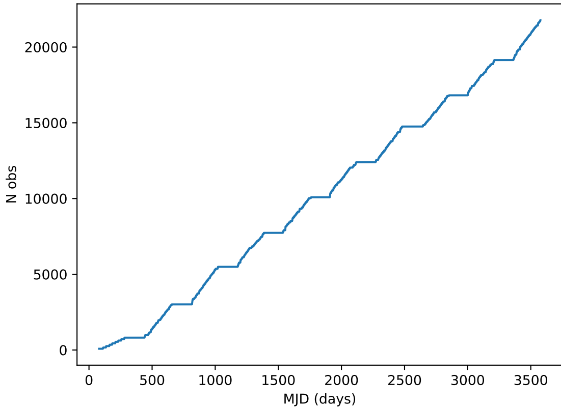
too_elab_heavy_r128_d2_ugrizy_v3.4_10yrs all bands: DD:XMM_LSS Cumulative NVisits
