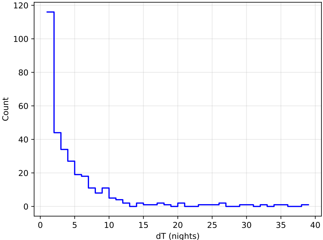
too_elab_heavy_r128_d2_ugrizy_v3.4_10yrs all bands: DD:WFD Delta Nights Histogram
