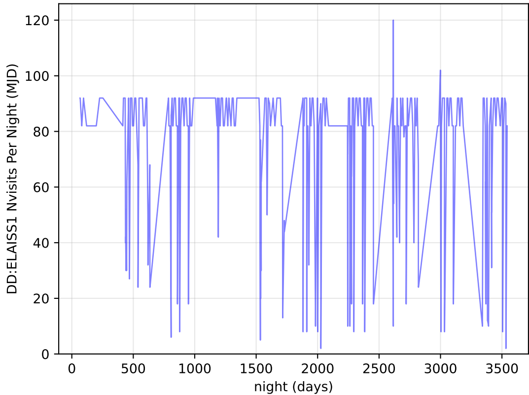
too_elab_heavy_r128_d2_ugrizy_v3.4_10yrs all bands: DD:ELAISS1 Nvisits Per Night
