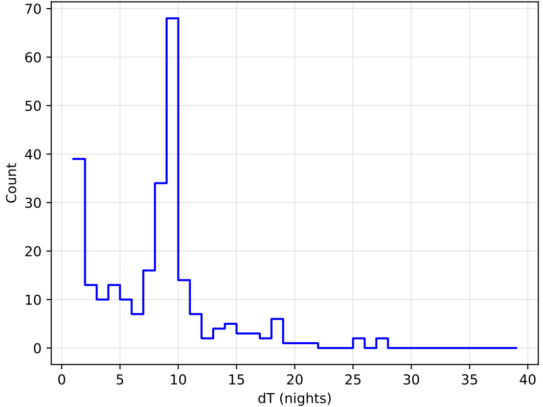
too_elab_heavy_r128_d2_ugrizy_v3.4_10yrs all bands: DD:ELAISS1 Delta Nights Histogram
