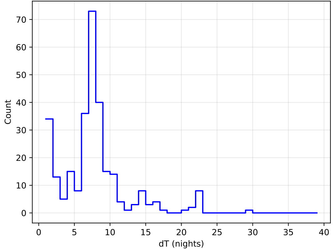
too_elab_heavy_r128_d2_ugrizy_v3.4_10yrs all bands: DD:EDFS Delta Nights Histogram
