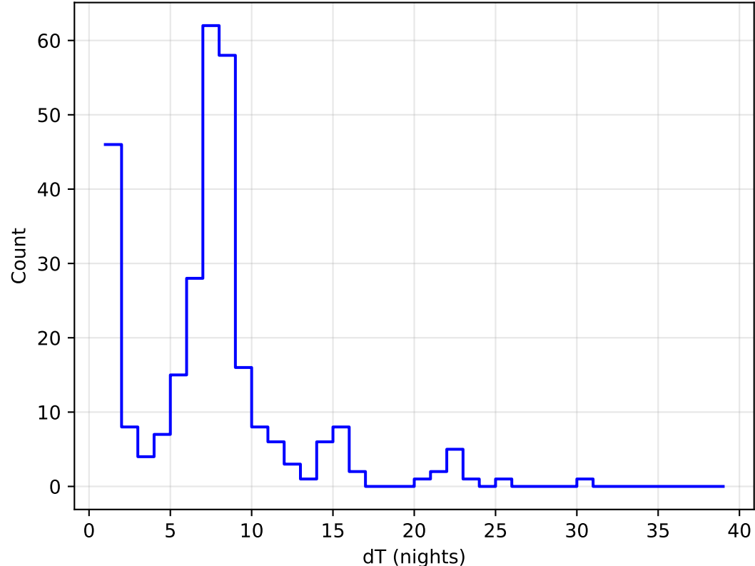
too_elab_heavy_r128_d2_ugrizy_v3.4_10yrs all bands: DD:ECDFS Delta Nights Histogram
